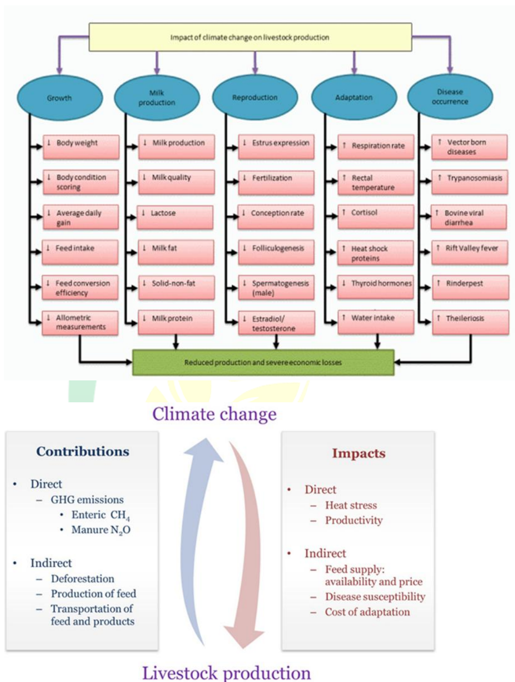
Fig.3. Impact of climate change on Livestock Production
