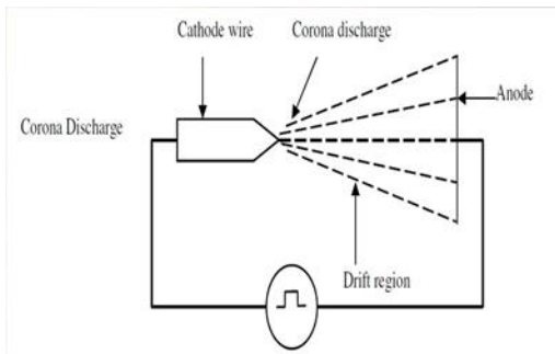
Fig 1 Corona discharge
