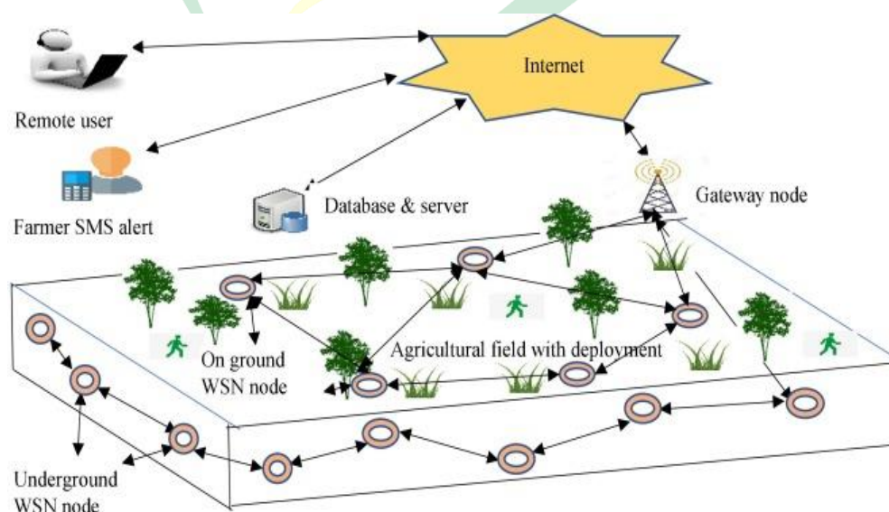
Figure 3: Wireless sensor network in agriculture
